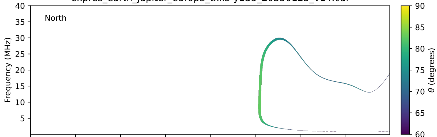
expres_earth_jupiter_europa_txka-y235_20350125_v14.cdf
