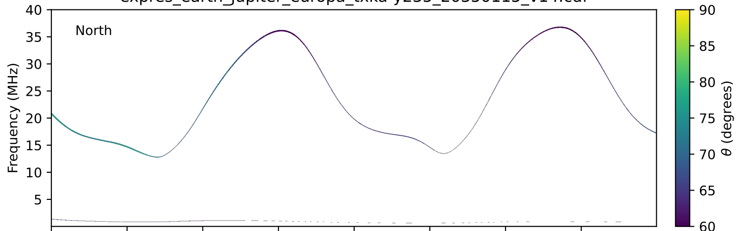
expres_earth_jupiter_europa_txka-y235_20350115_v14.cdf
