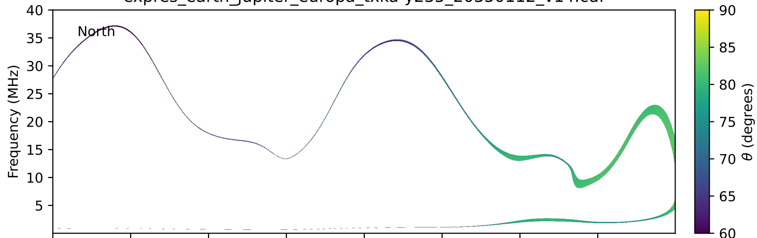
expres_earth_jupiter_europa_txka-y235_20350112_v14.cdf
