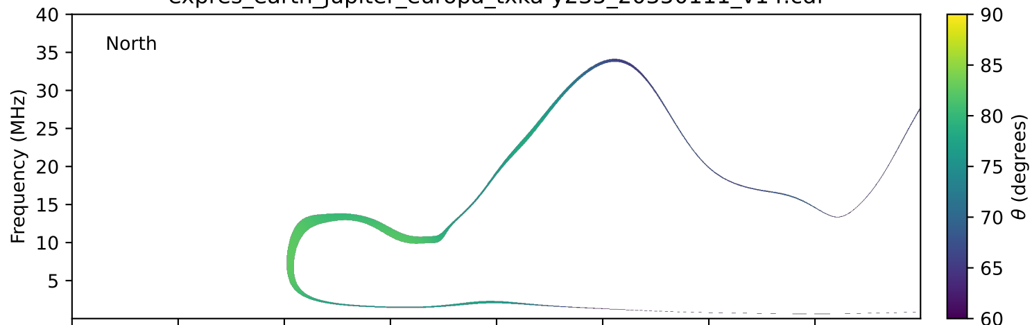
expres_earth_jupiter_europa_txka-y235_20350111_v14.cdf
