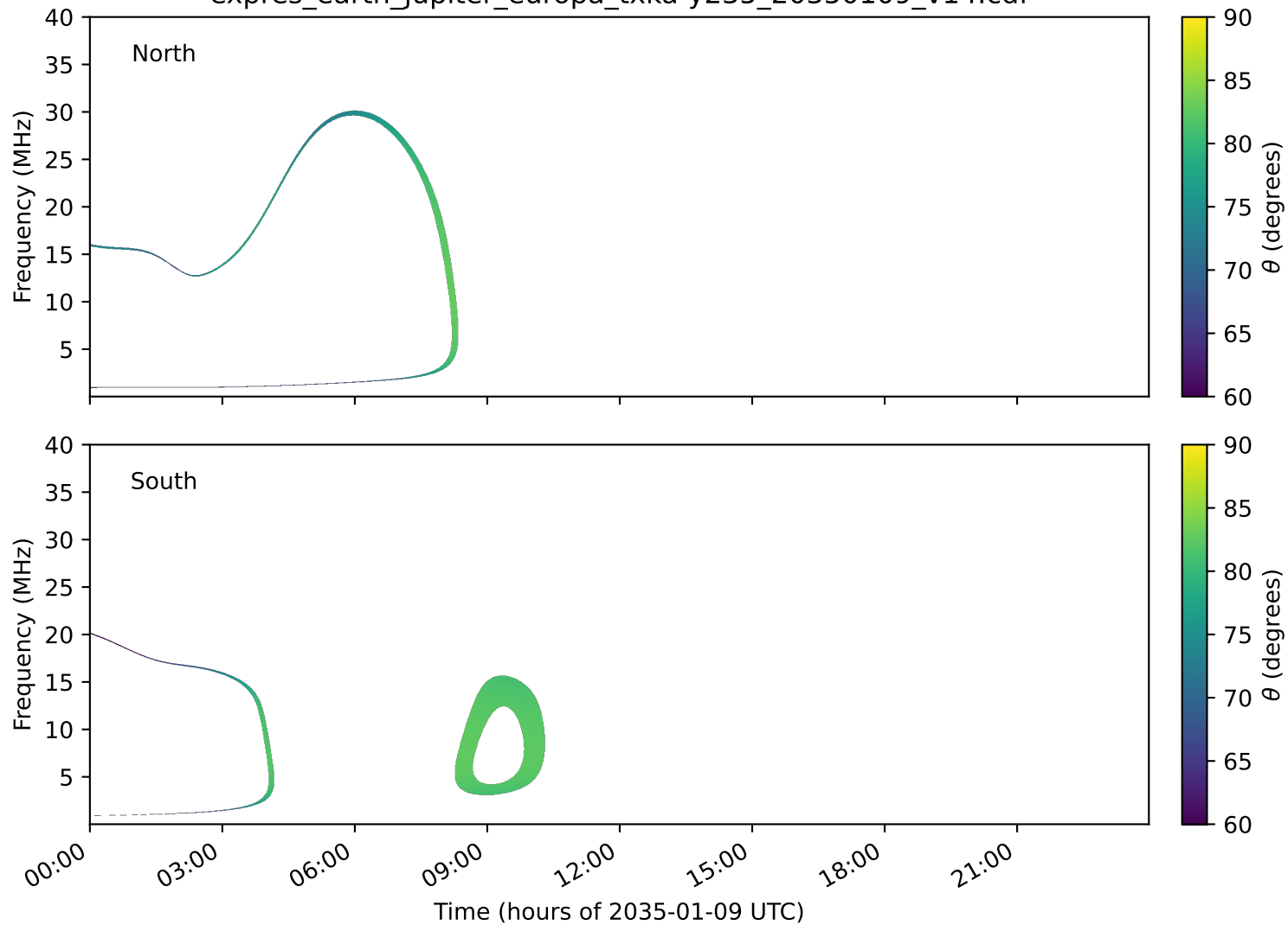
expres_earth_jupiter_europa_txka-y235_20350109_v14.cdf
