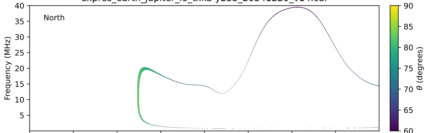
expres_earth_jupiter_io_txka-y235_20341220_v14.cdf
