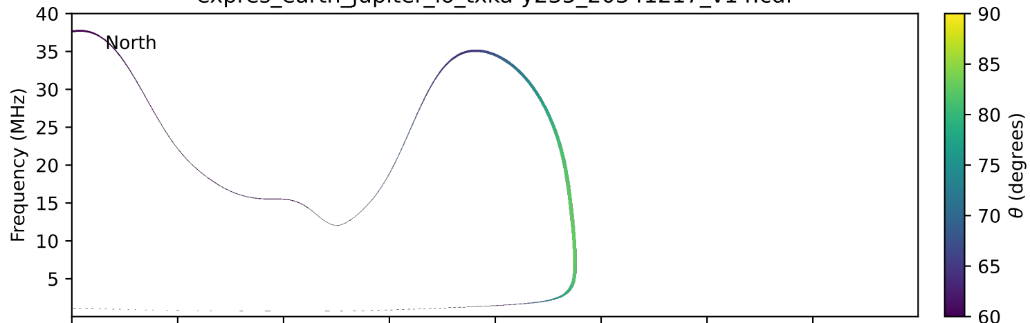
expres_earth_jupiter_io_txka-y235_20341217_v14.cdf
