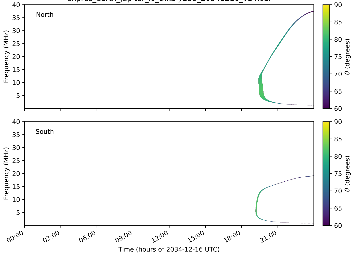
expres_earth_jupiter_io_txka-y235_20341216_v14.cdf
