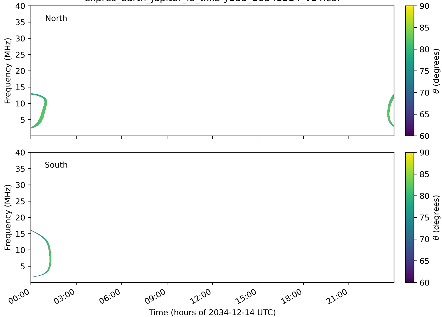
expres_earth_jupiter_io_txka-y235_20341214_v14.cdf
