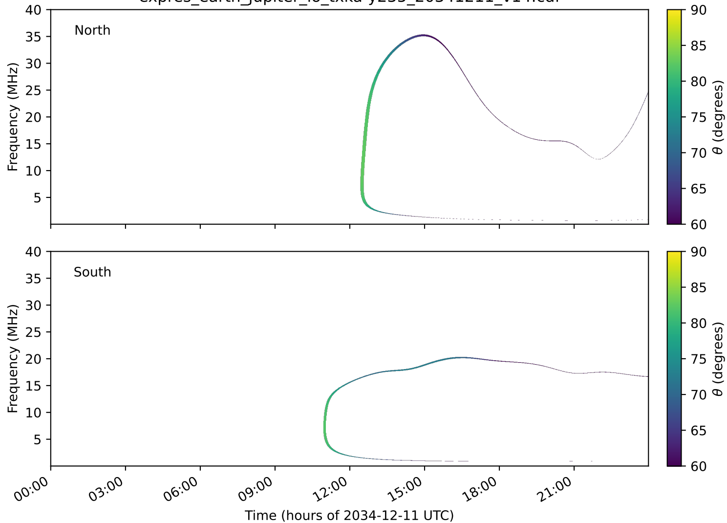
expres_earth_jupiter_io_txka-y235_20341211_v14.cdf
