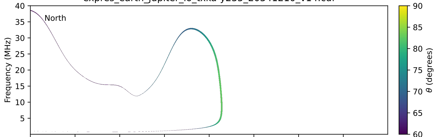
expres_earth_jupiter_io_txka-y235_20341210_v14.cdf
