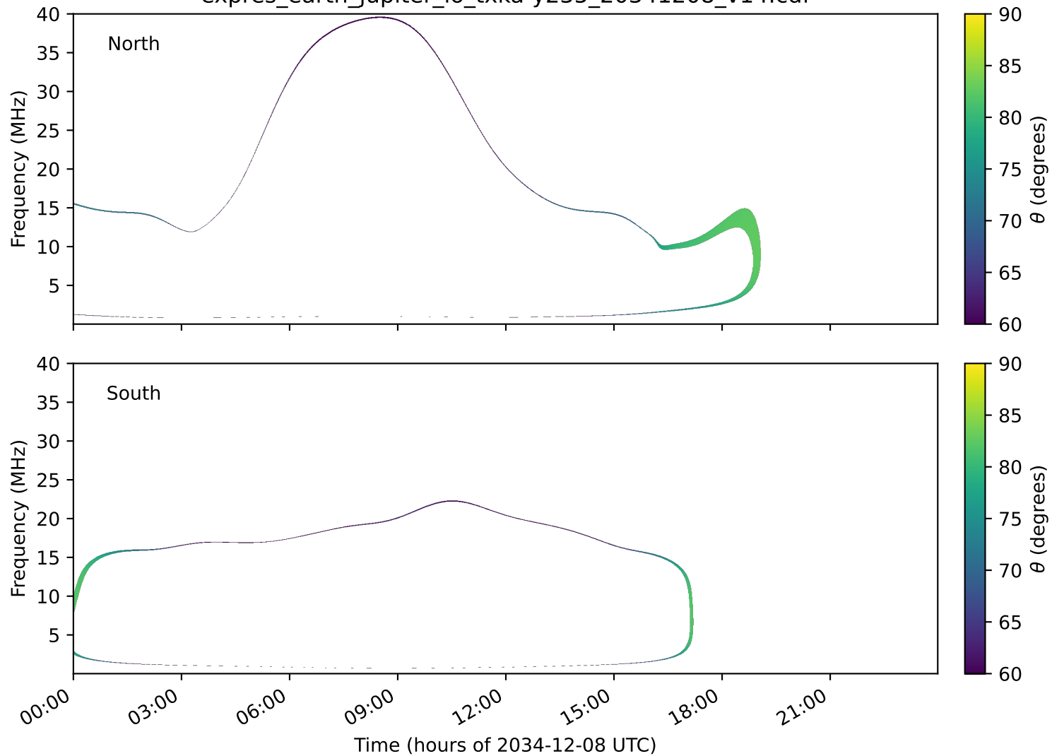
expres_earth_jupiter_io_txka-y235_20341208_v14.cdf
