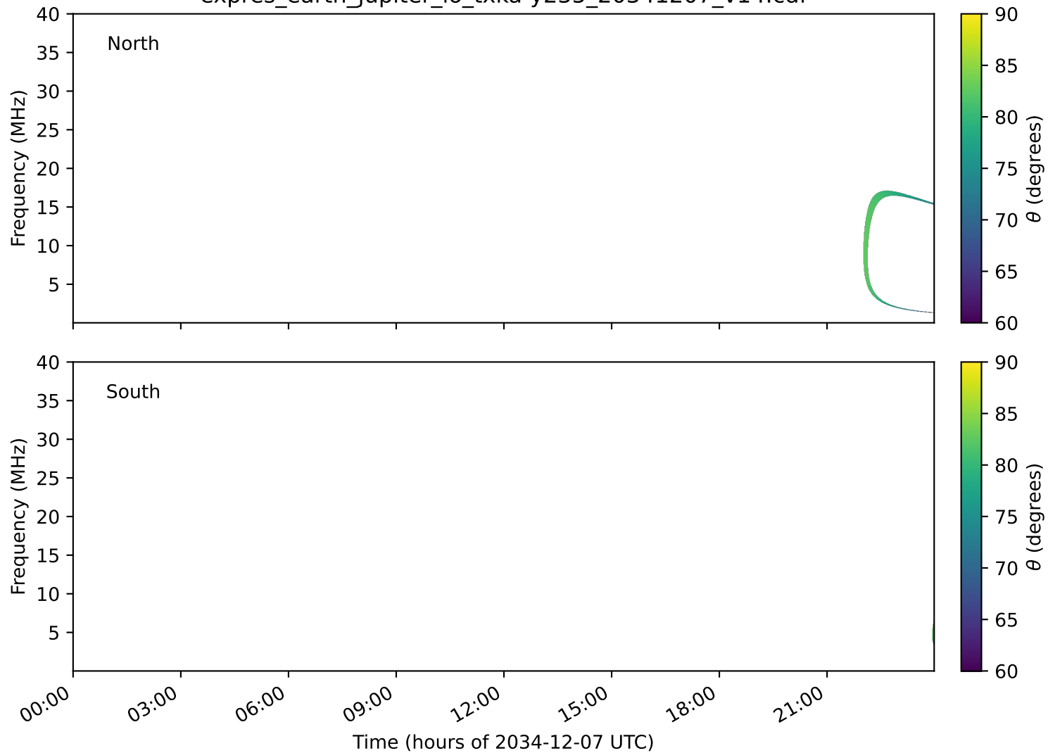
expres_earth_jupiter_io_txka-y235_20341207_v14.cdf
