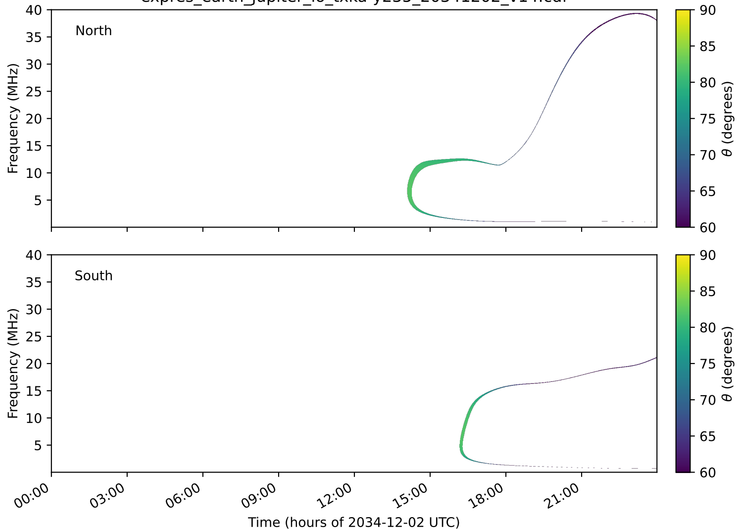
expres_earth_jupiter_io_txka-y235_20341202_v14.cdf
