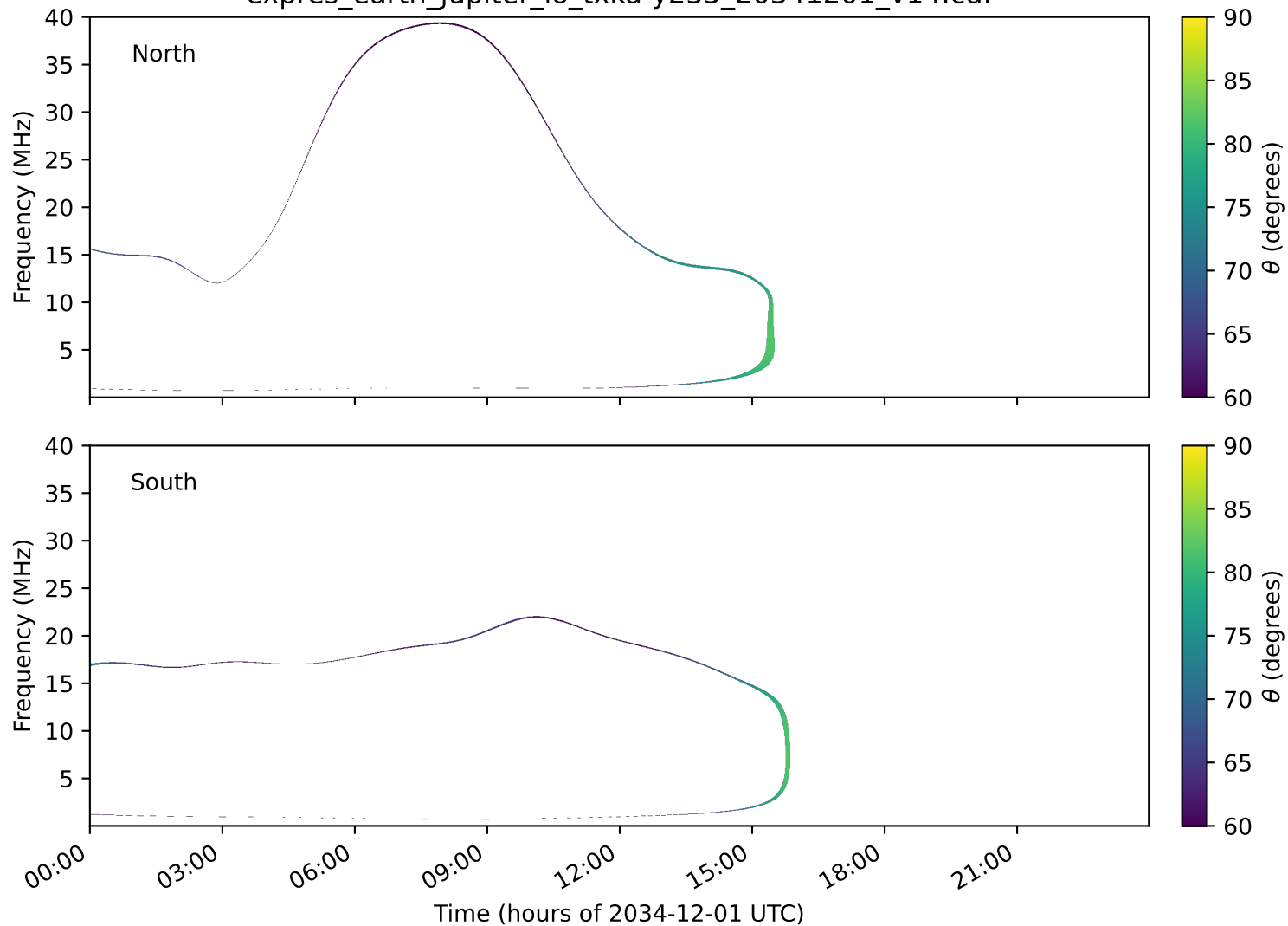
expres_earth_jupiter_io_txka-y235_20341201_v14.cdf
