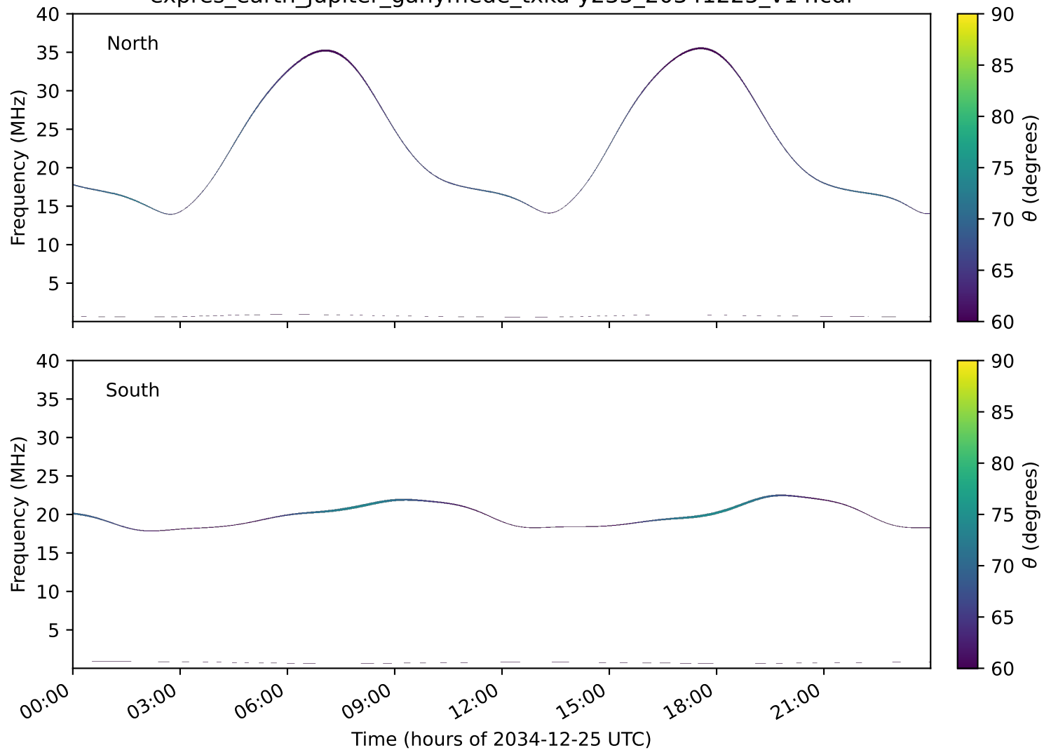
expres_earth_jupiter_ganymede_txka-y235_20341225_v14.cdf
