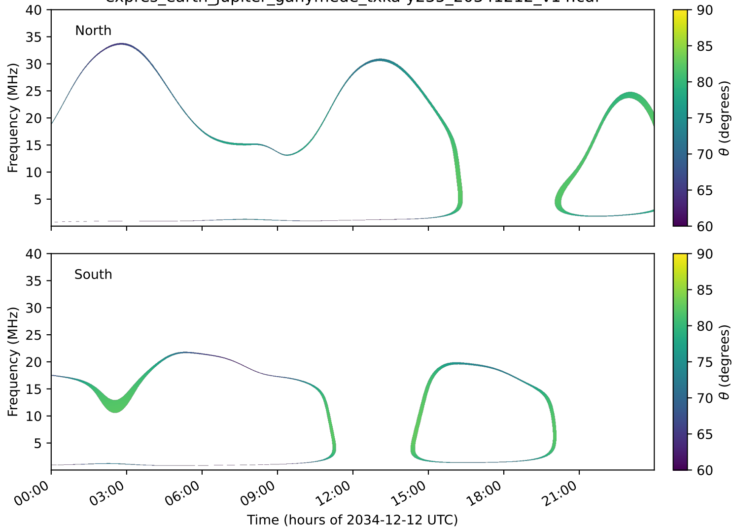
expres_earth_jupiter_ganymede_txka-y235_20341212_v14.cdf
