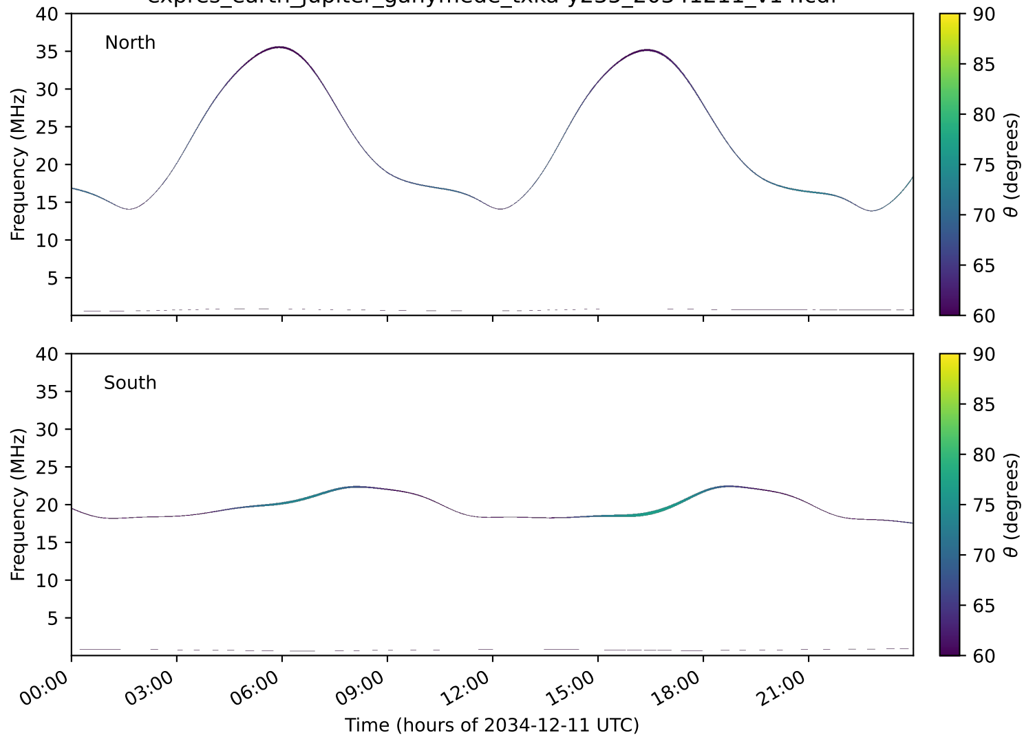
expres_earth_jupiter_ganymede_txka-y235_20341211_v14.cdf
