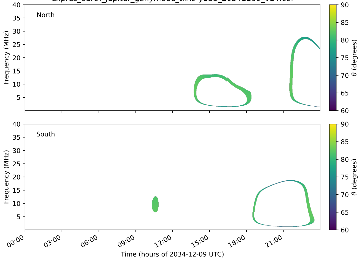
expres_earth_jupiter_ganymede_txka-y235_20341209_v14.cdf
