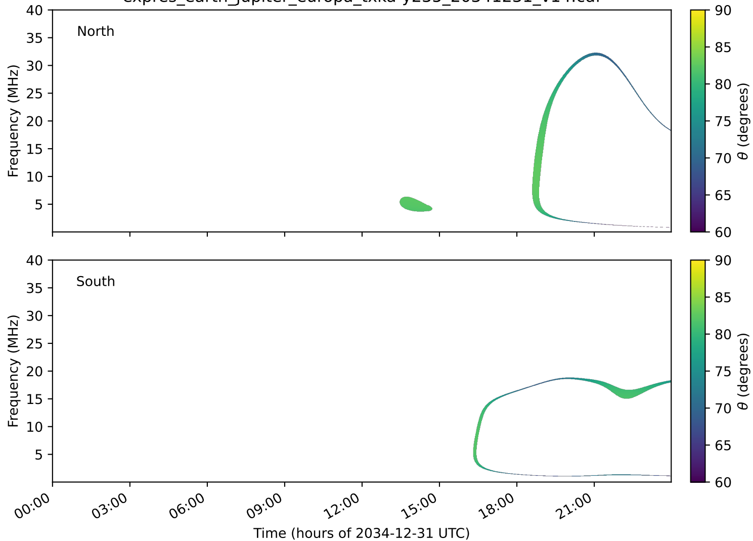
expres_earth_jupiter_europa_txka-y235_20341231_v14.cdf
