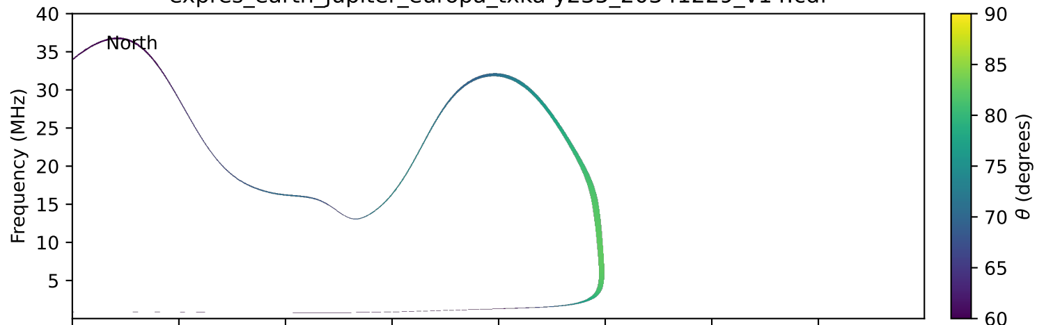
expres_earth_jupiter_europa_txka-y235_20341229_v14.cdf
