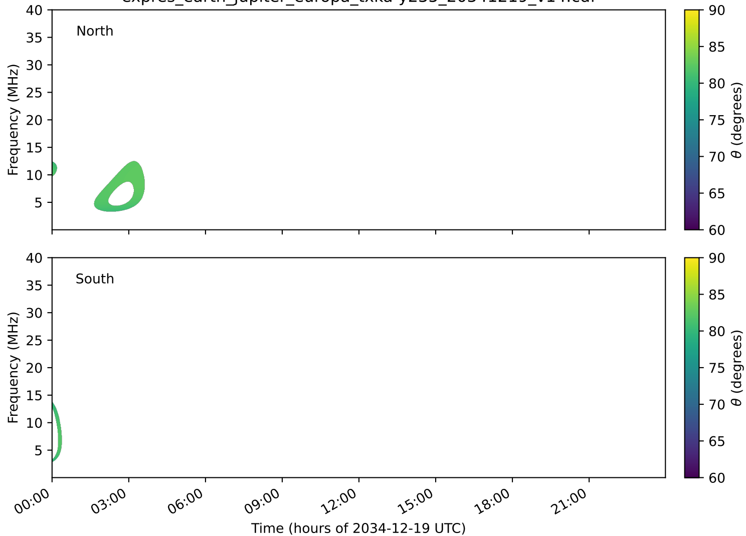
expres_earth_jupiter_europa_txka-y235_20341219_v14.cdf
