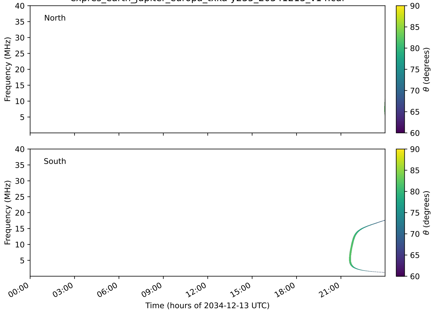
expres_earth_jupiter_europa_txka-y235_20341213_v14.cdf
