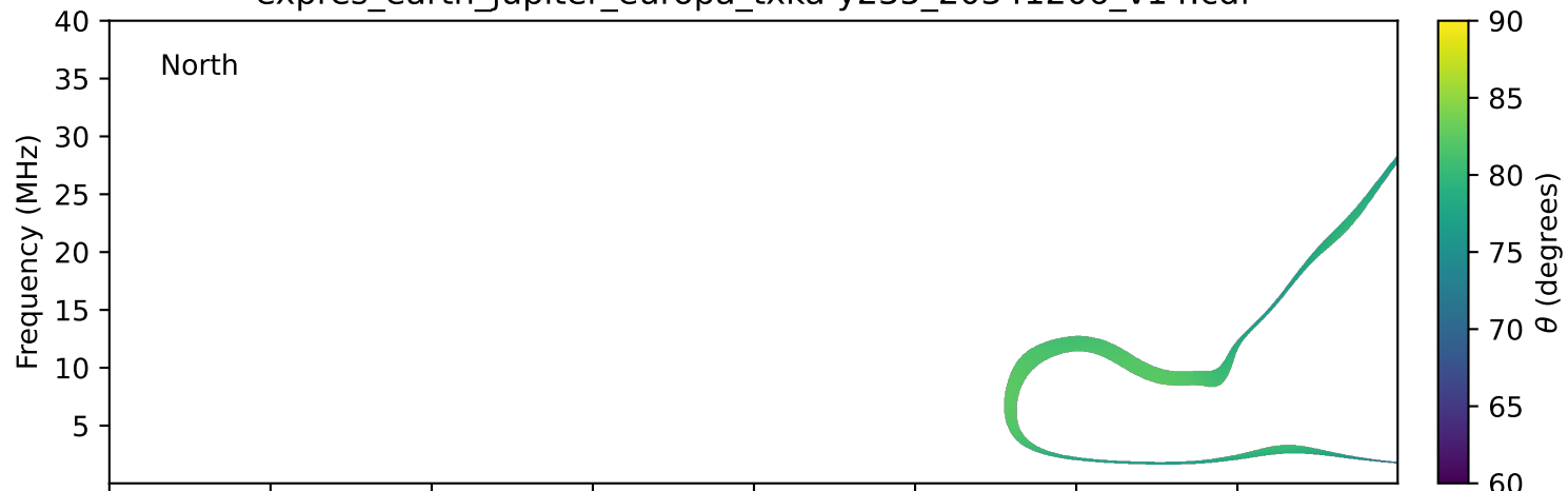
expres_earth_jupiter_europa_txka-y235_20341206_v14.cdf
