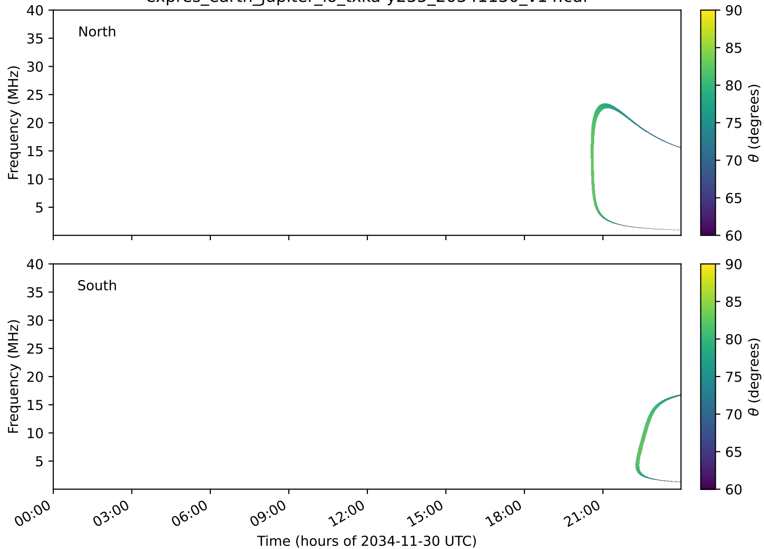
expres_earth_jupiter_io_txka-y235_20341130_v14.cdf
