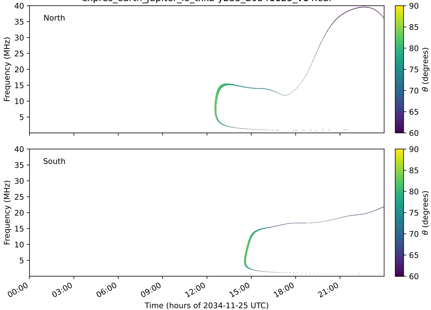
expres_earth_jupiter_io_txka-y235_20341125_v14.cdf
