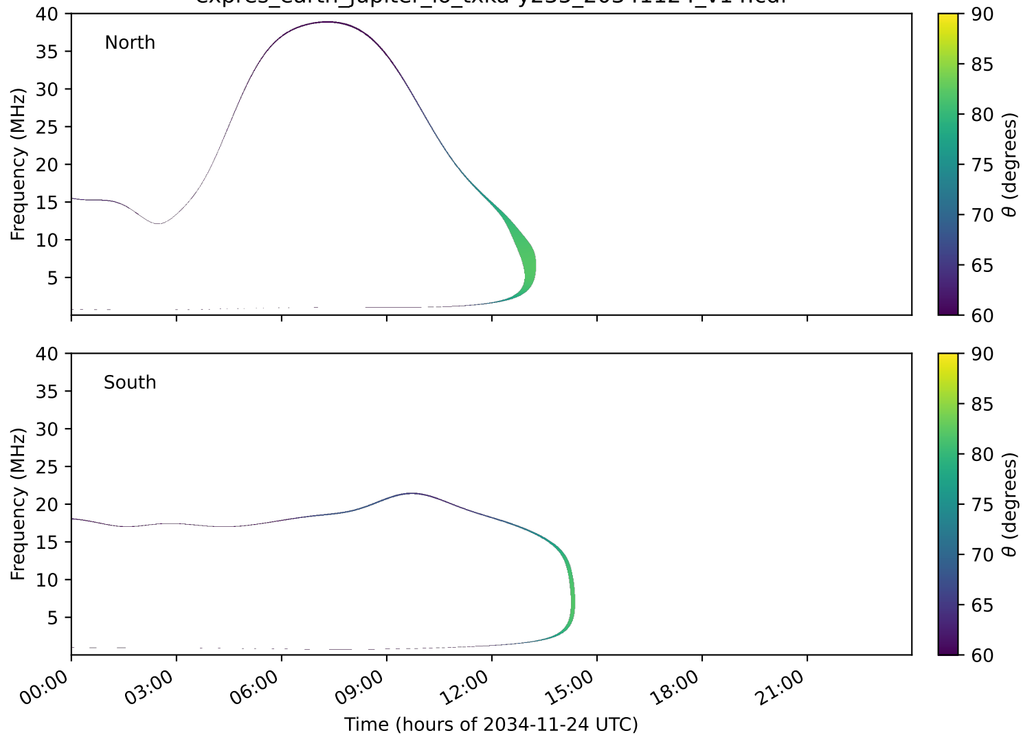
expres_earth_jupiter_io_txka-y235_20341124_v14.cdf
