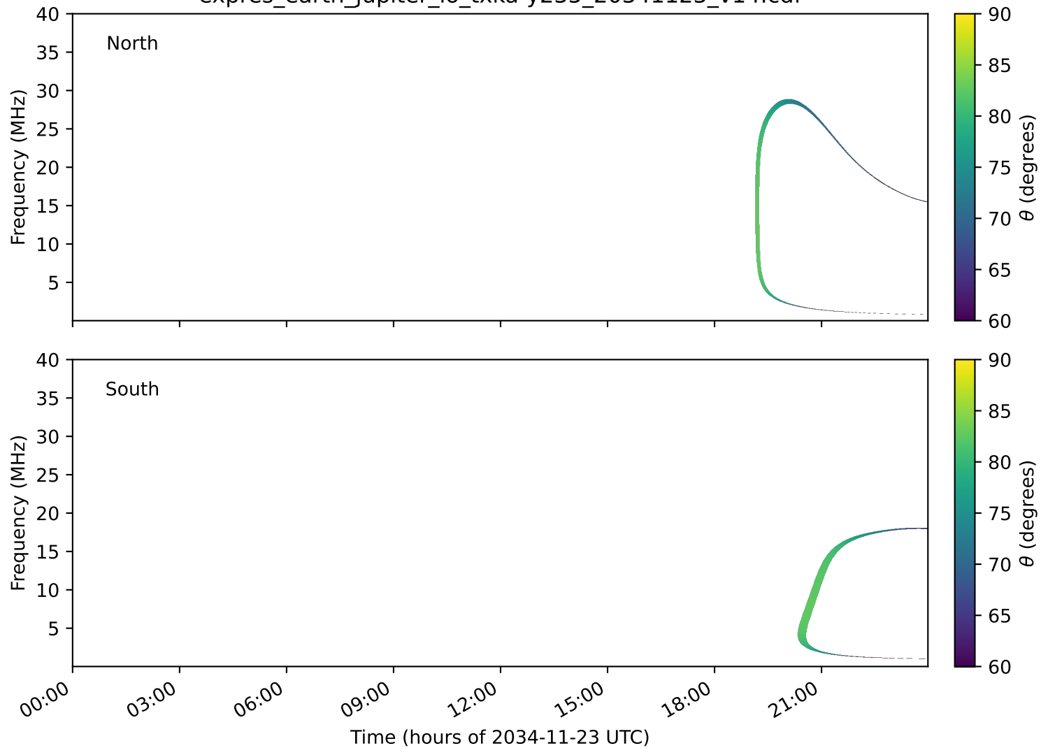
expres_earth_jupiter_io_txka-y235_20341123_v14.cdf
