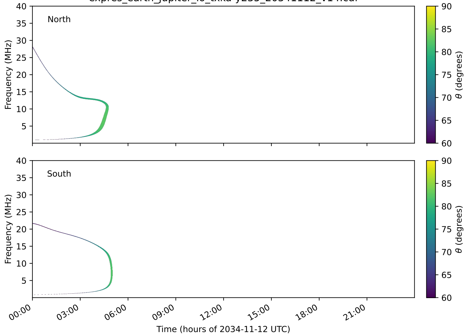
expres_earth_jupiter_io_txka-y235_20341112_v14.cdf
