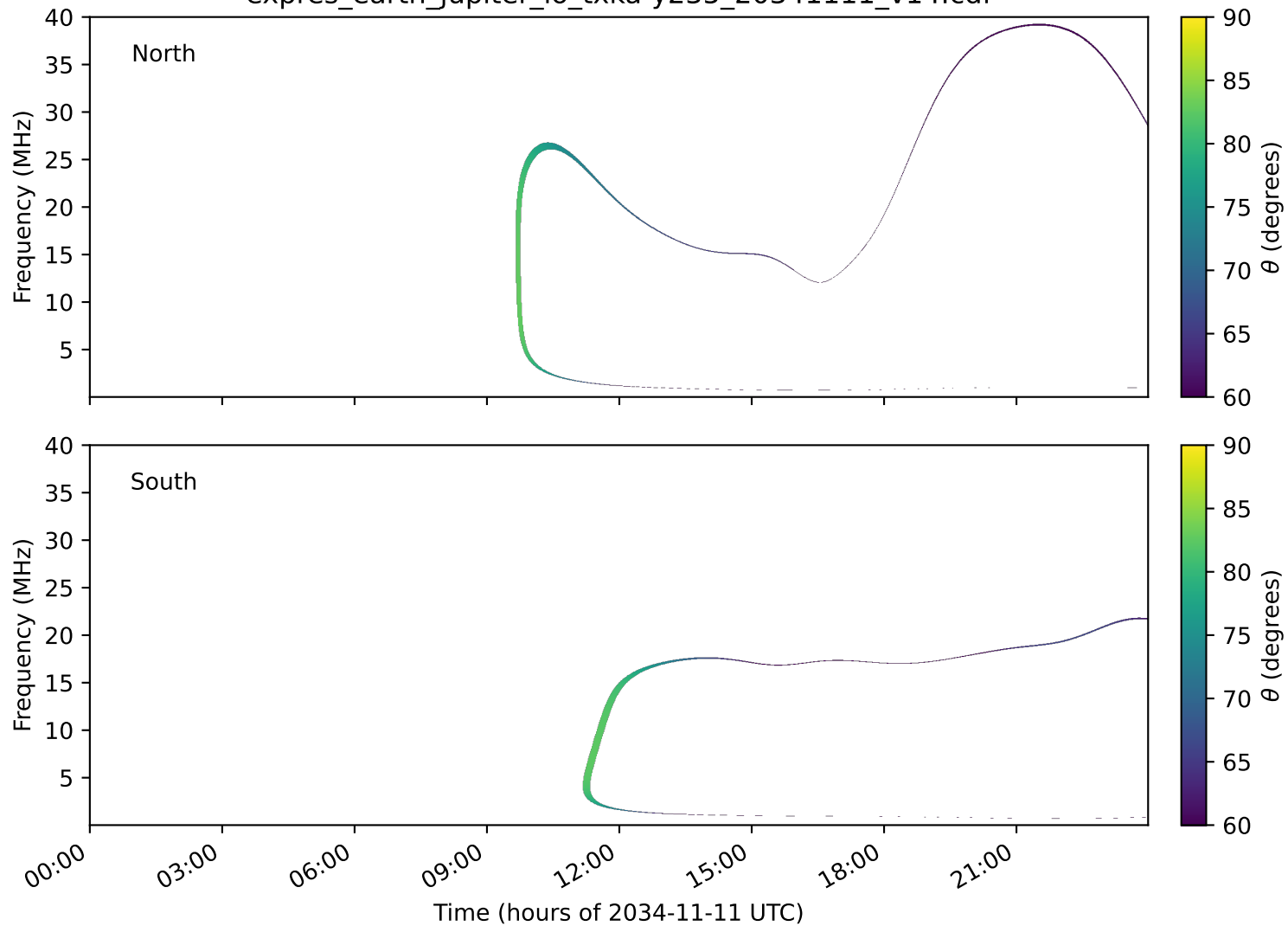
expres_earth_jupiter_io_txka-y235_20341111_v14.cdf
