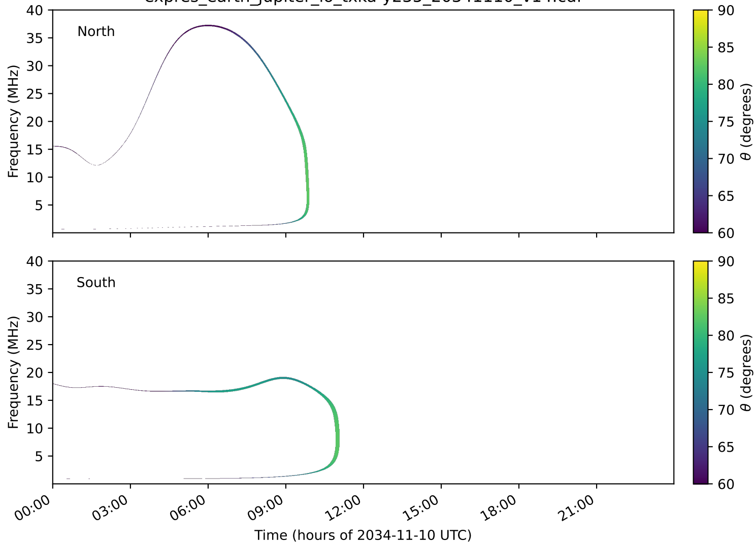
expres_earth_jupiter_io_txka-y235_20341110_v14.cdf
