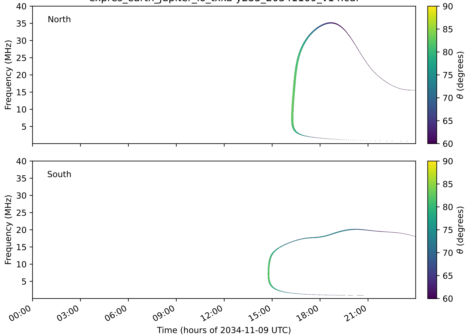
expres_earth_jupiter_io_txka-y235_20341109_v14.cdf
