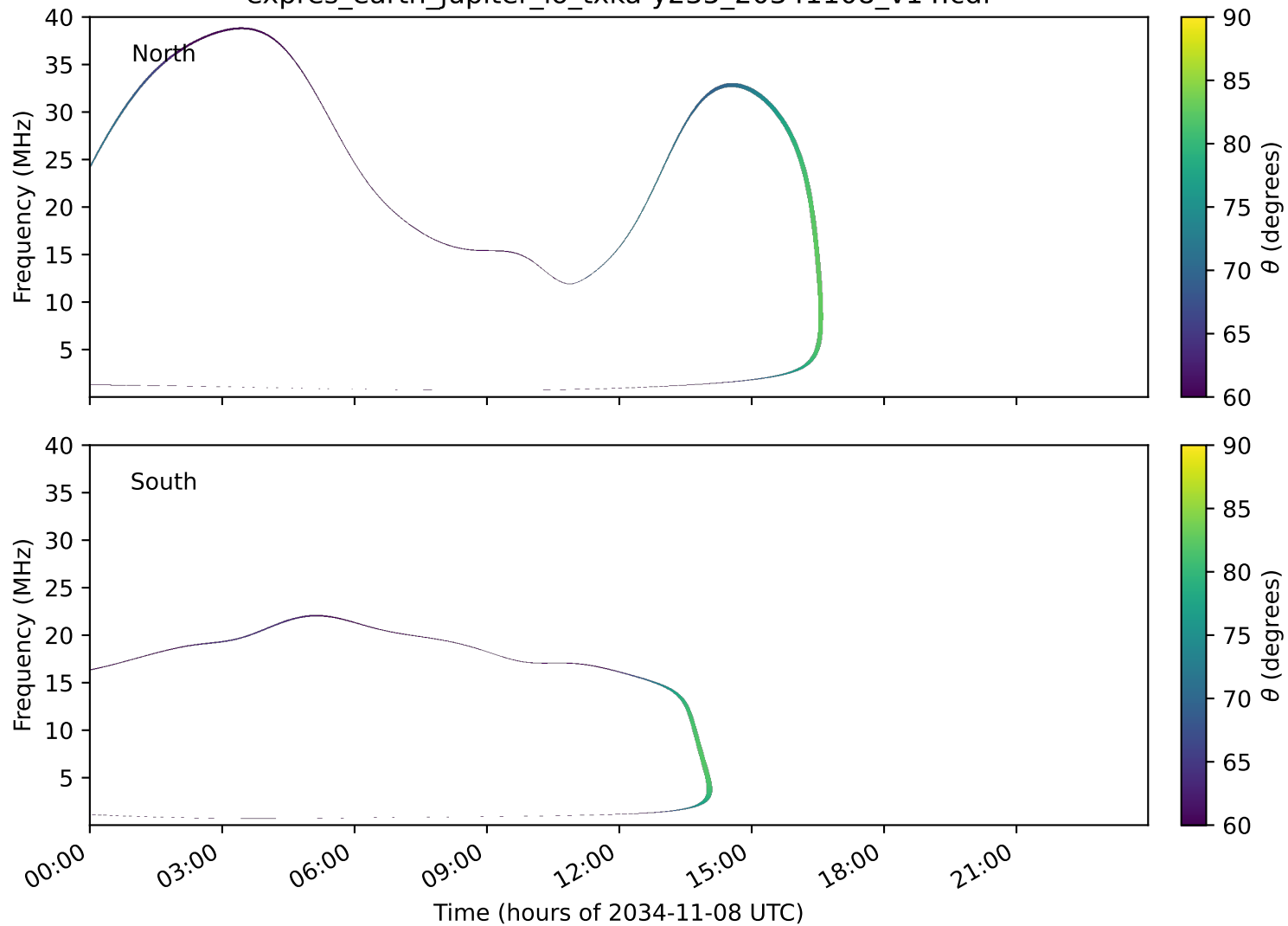
expres_earth_jupiter_io_txka-y235_20341108_v14.cdf
