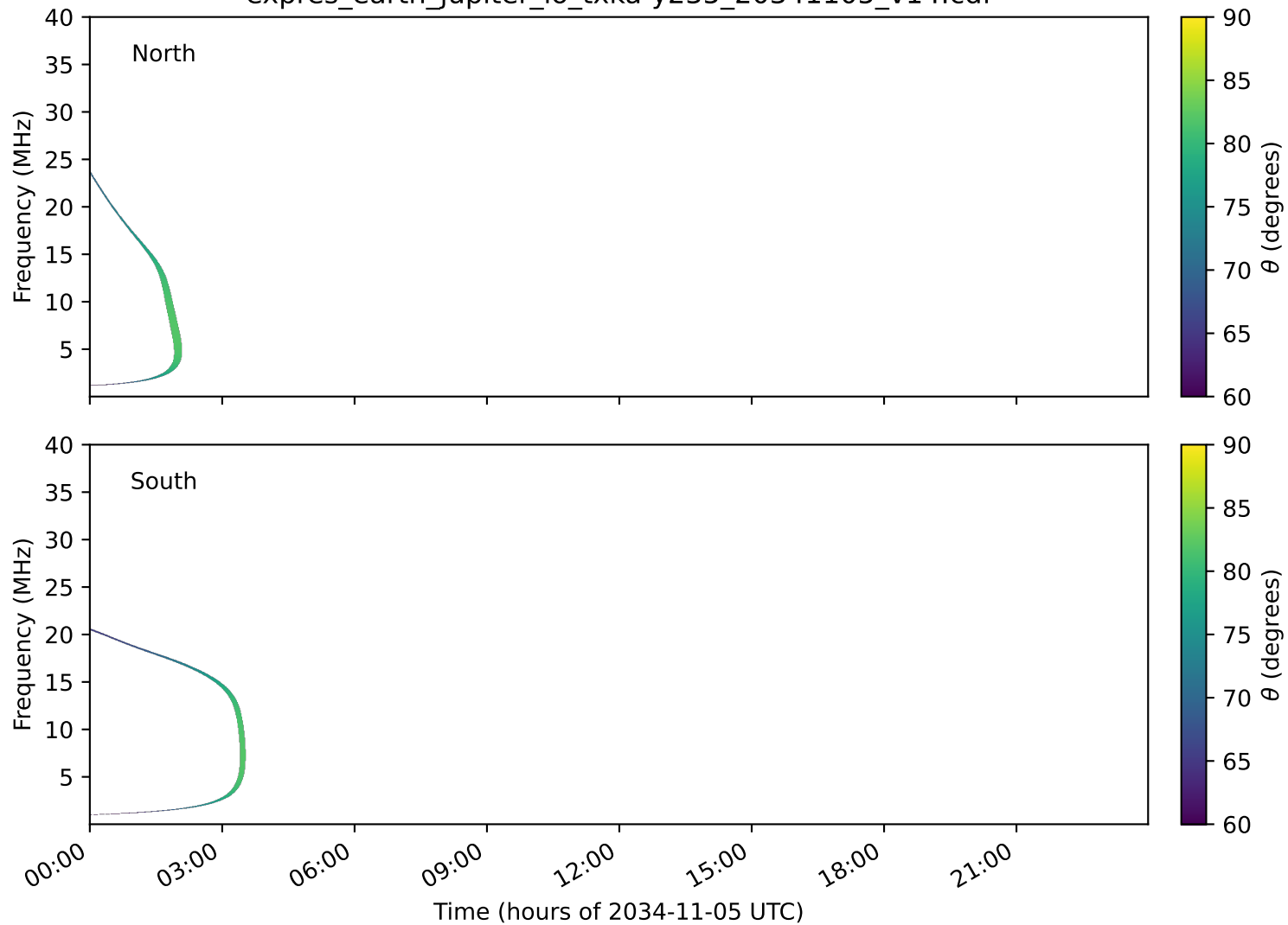
expres_earth_jupiter_io_txka-y235_20341105_v14.cdf
