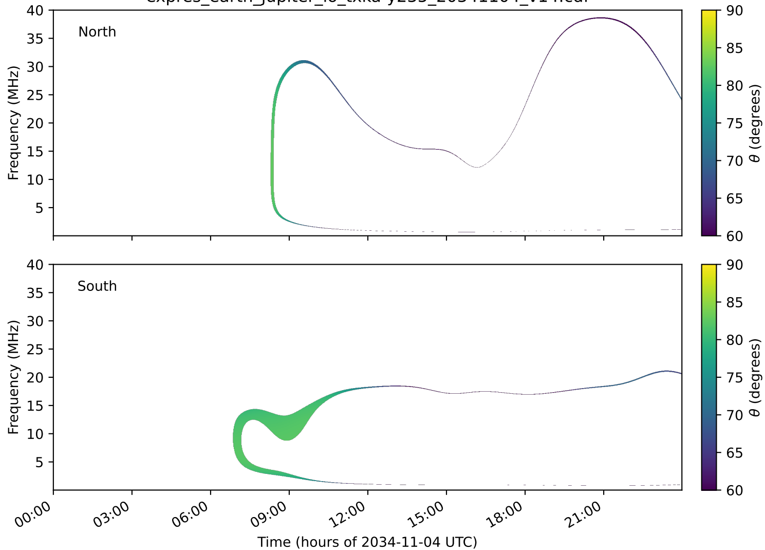
expres_earth_jupiter_io_txka-y235_20341104_v14.cdf
