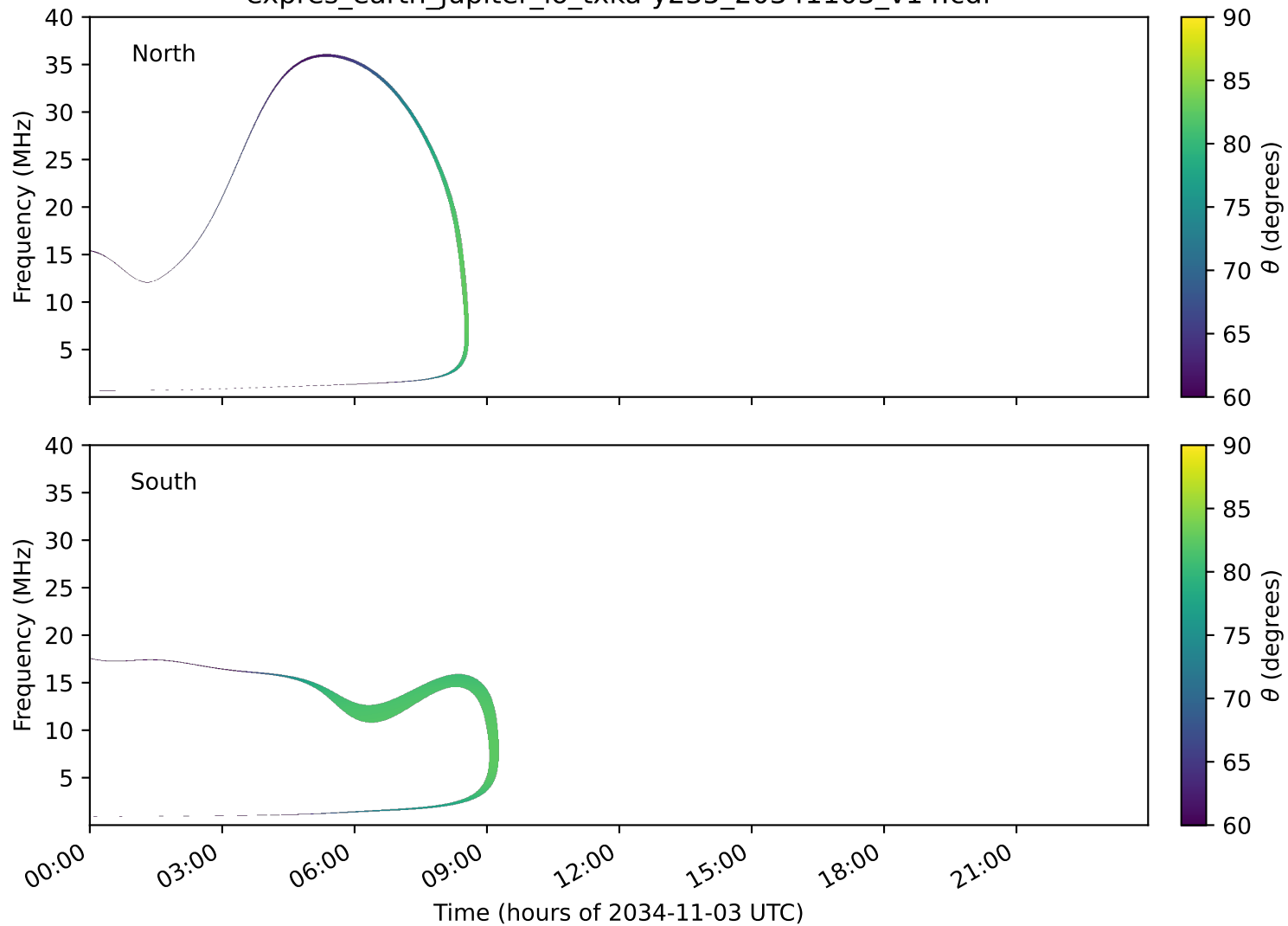
expres_earth_jupiter_io_txka-y235_20341103_v14.cdf
