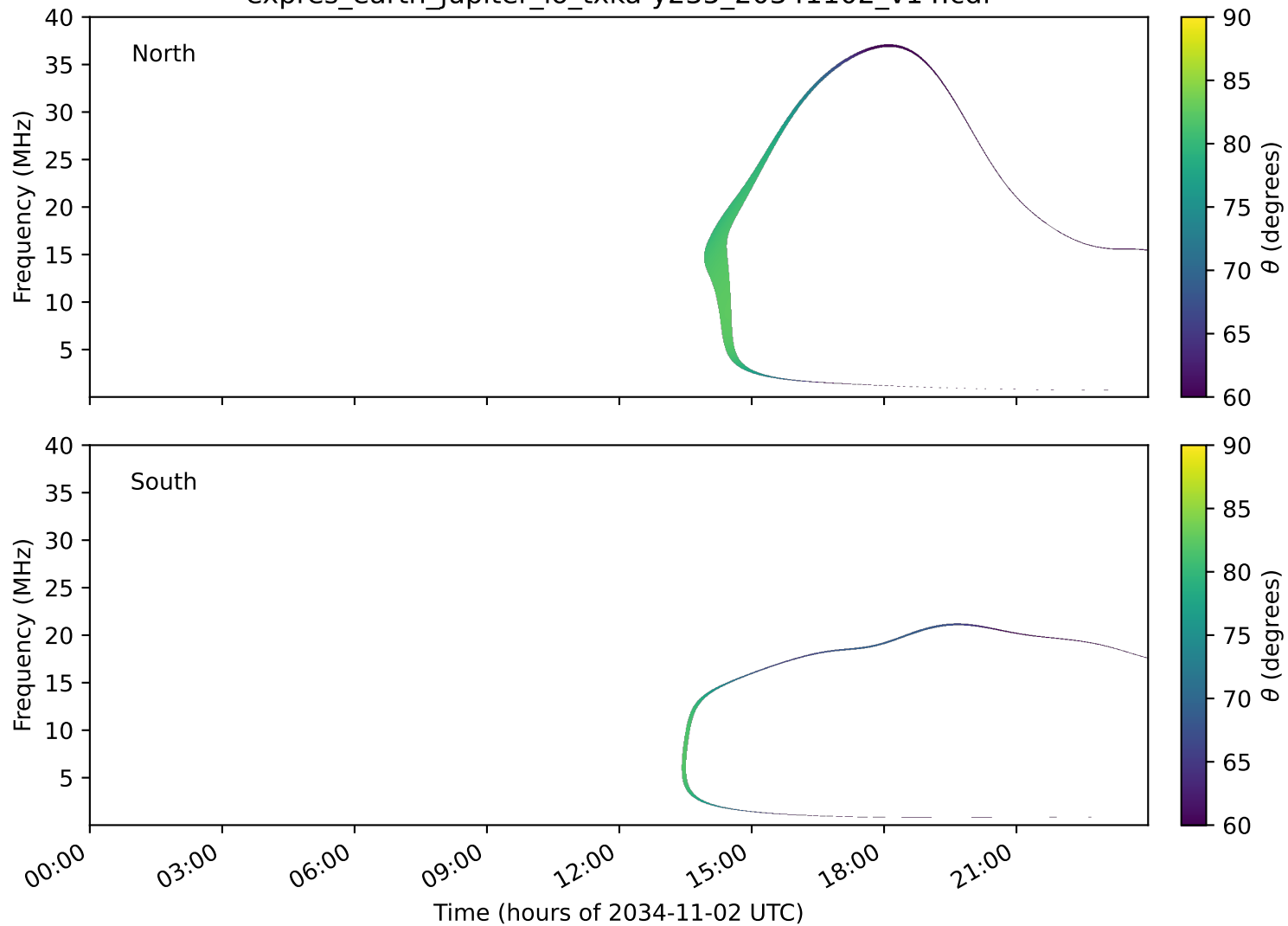
expres_earth_jupiter_io_txka-y235_20341102_v14.cdf
