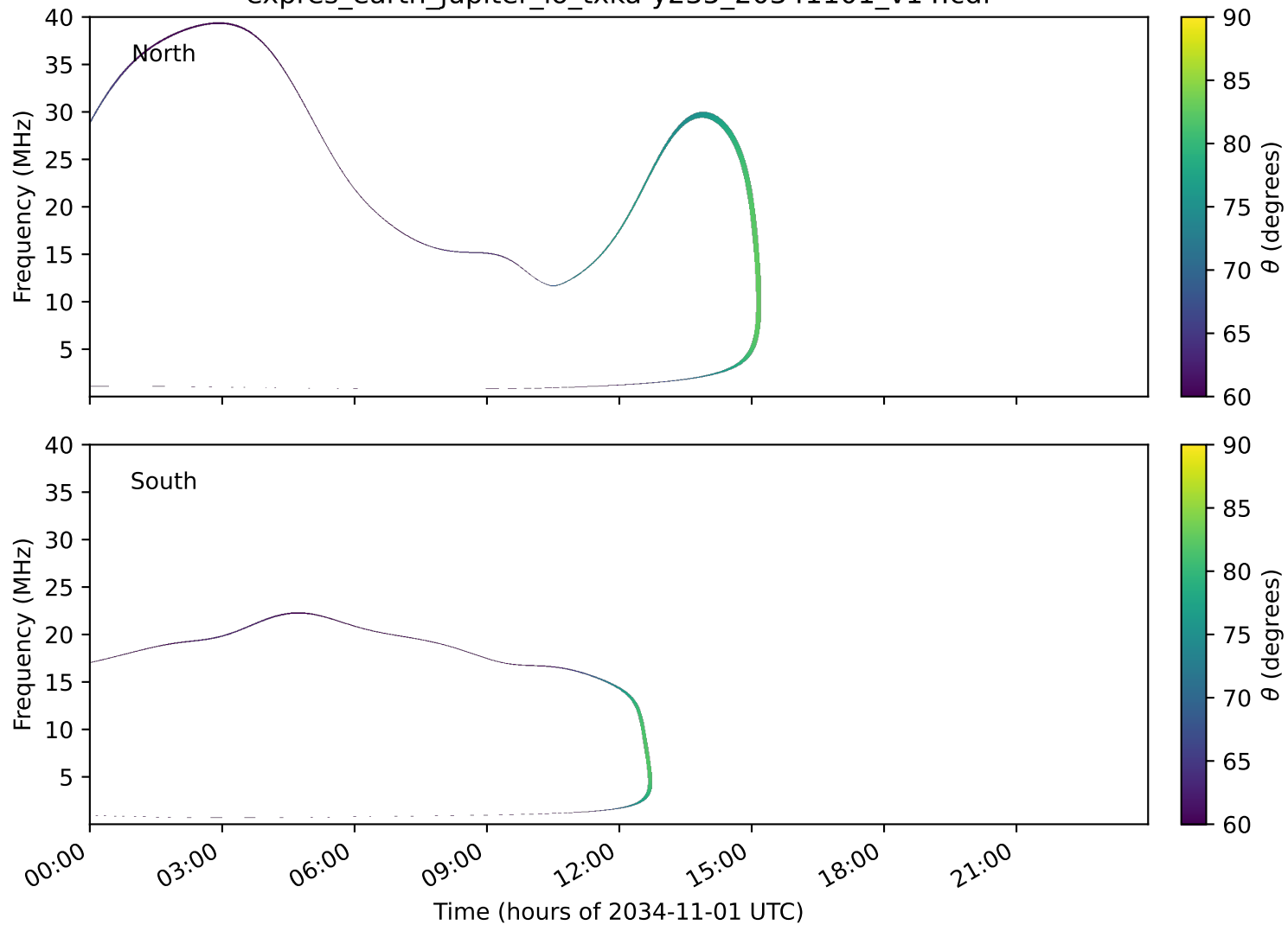
expres_earth_jupiter_io_txka-y235_20341101_v14.cdf
