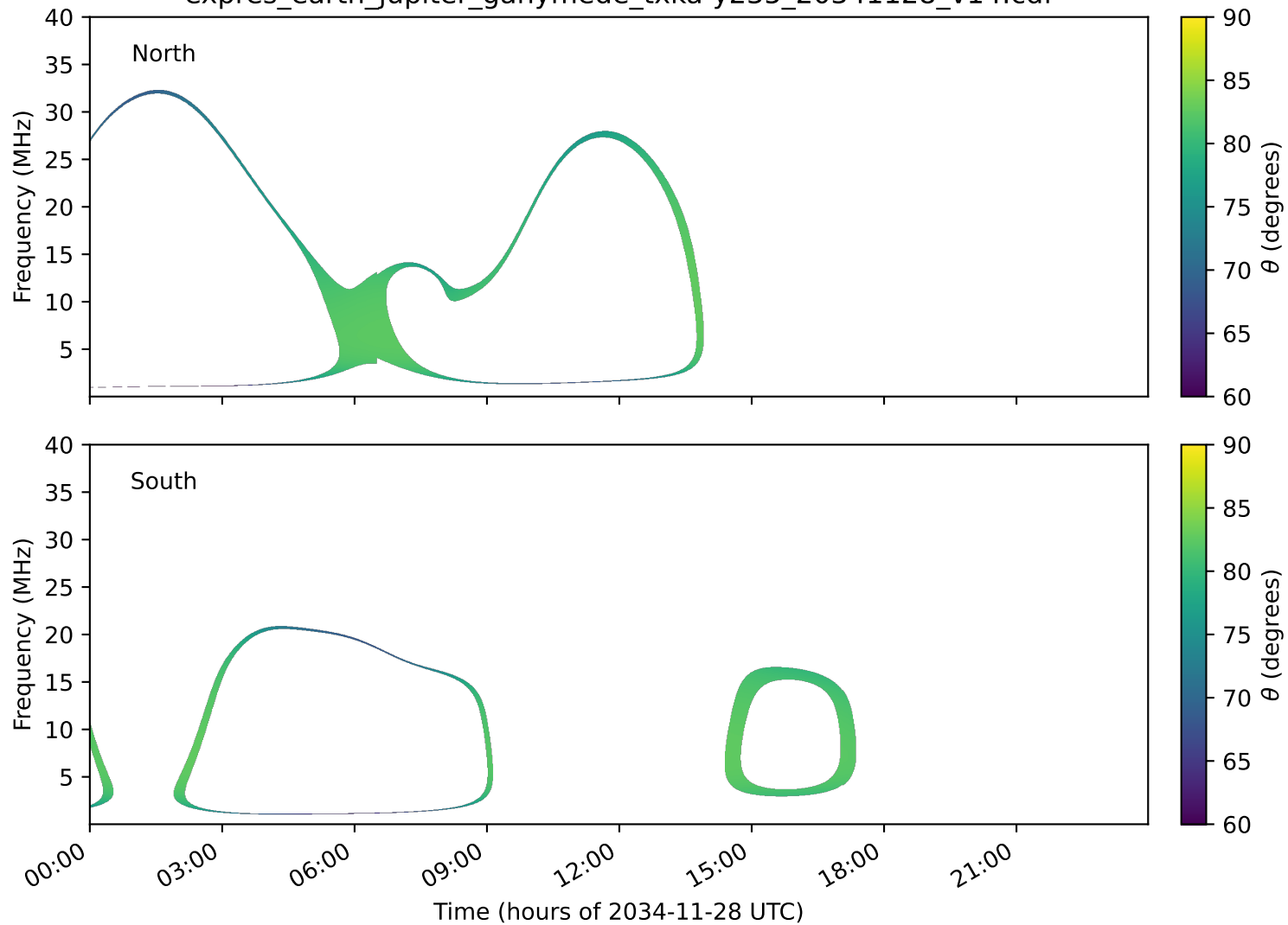
expres_earth_jupiter_ganymede_txka-y235_20341128_v14.cdf
