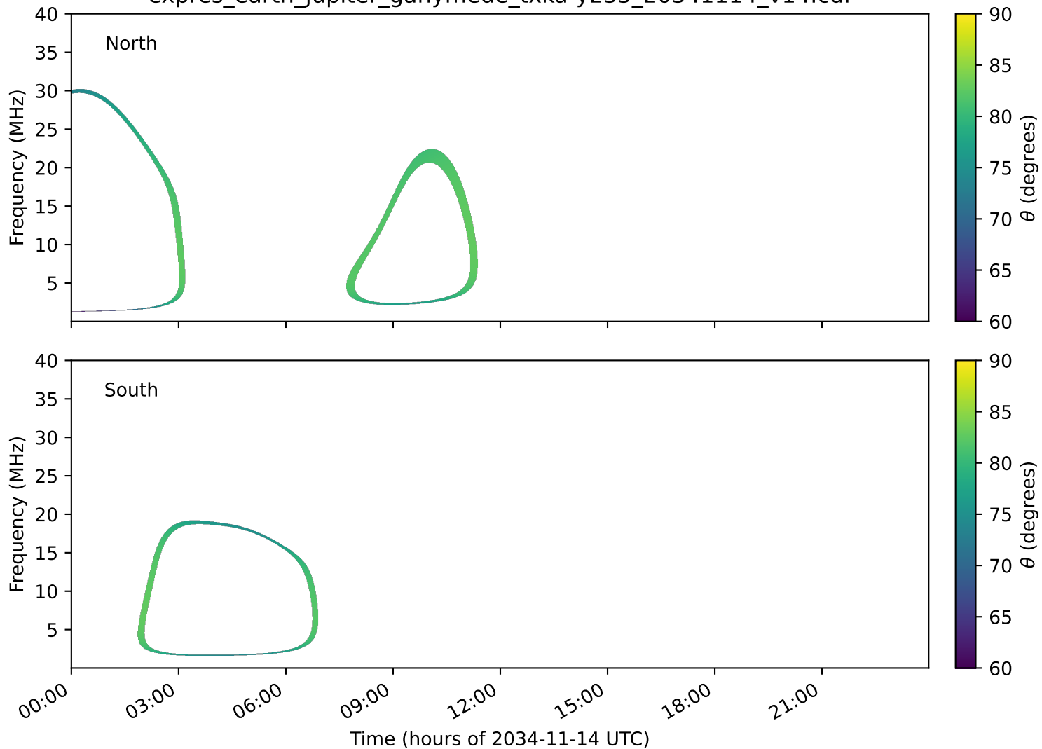
expres_earth_jupiter_ganymede_txka-y235_20341114_v14.cdf
