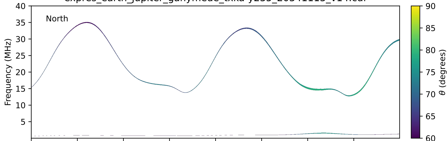
expres_earth_jupiter_ganymede_txka-y235_20341113_v14.cdf
