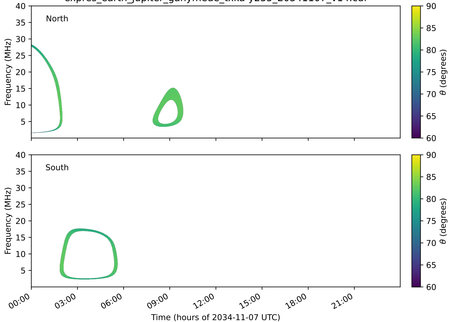
expres_earth_jupiter_ganymede_txka-y235_20341107_v14.cdf
