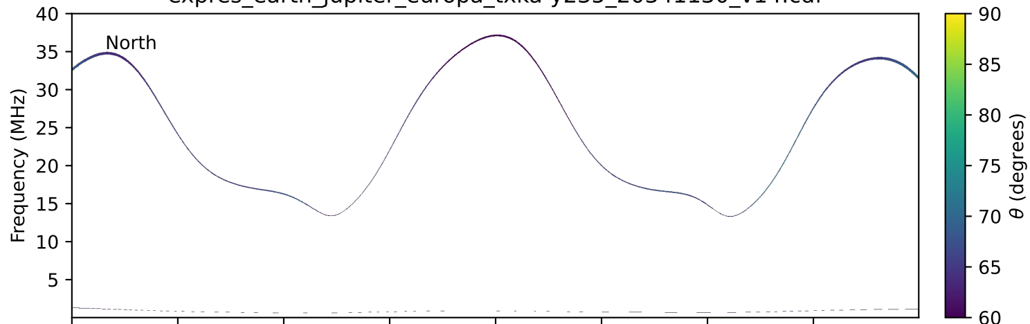
expres_earth_jupiter_europa_txka-y235_20341130_v14.cdf
