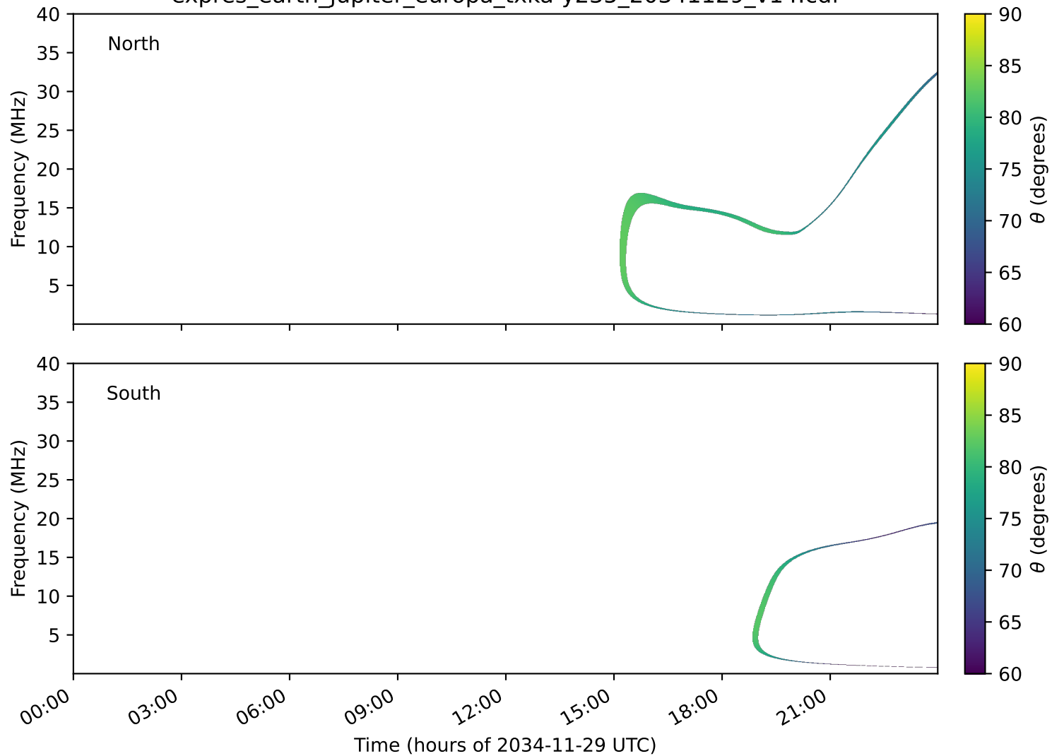
expres_earth_jupiter_europa_txka-y235_20341129_v14.cdf
