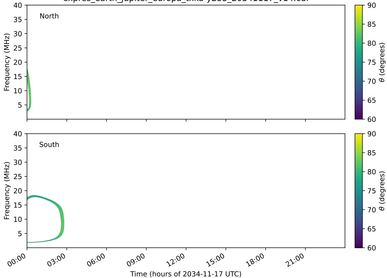
expres_earth_jupiter_europa_txka-y235_20341117_v14.cdf
