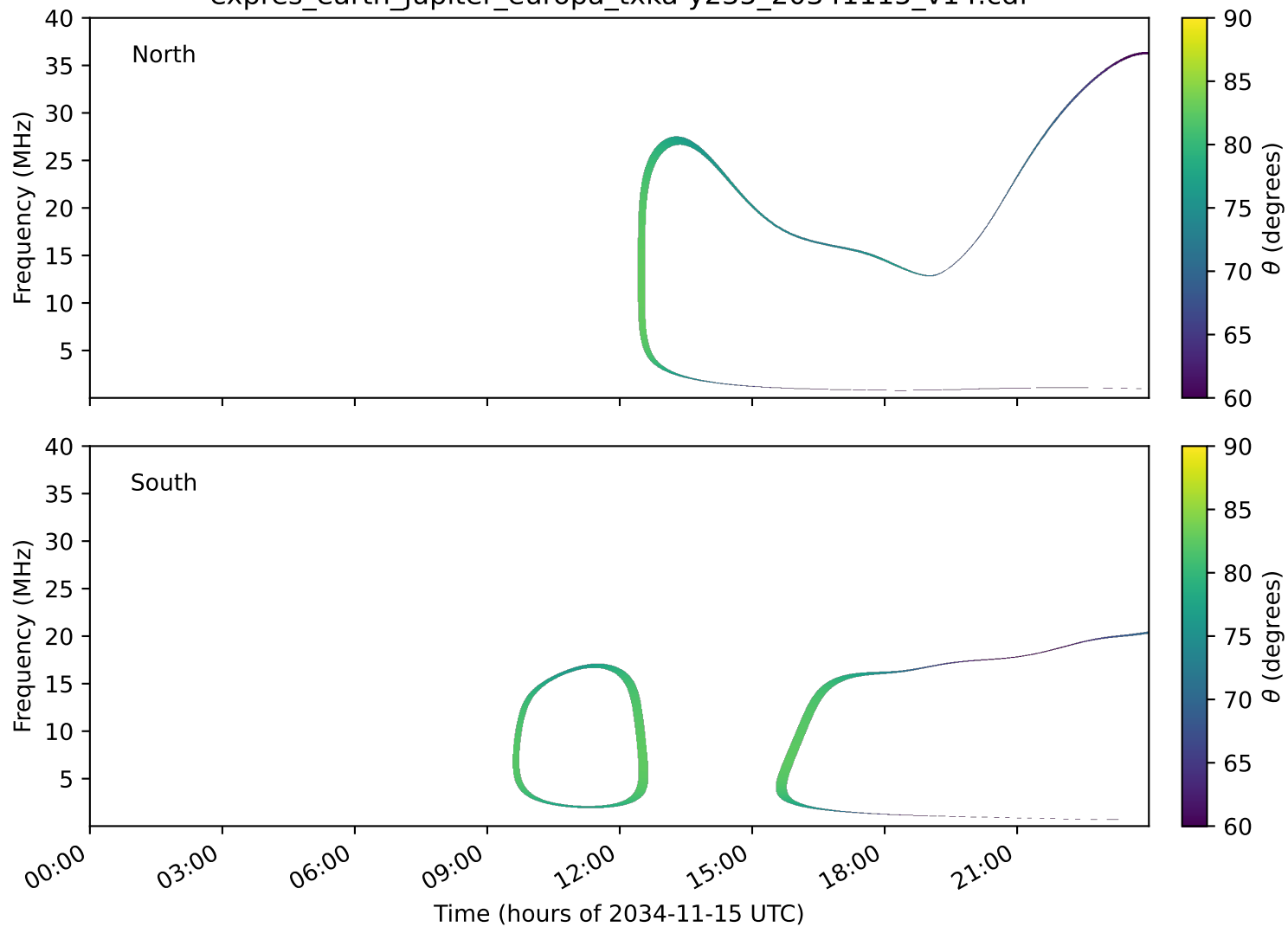
expres_earth_jupiter_europa_txka-y235_20341115_v14.cdf
