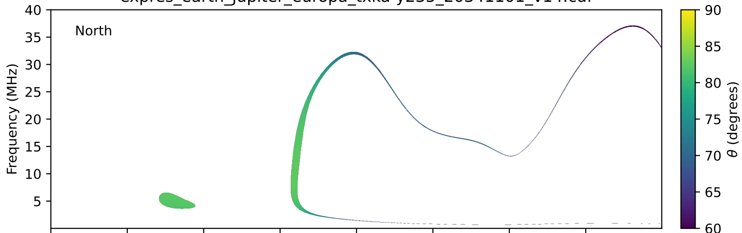
expres_earth_jupiter_europa_txka-y235_20341101_v14.cdf
