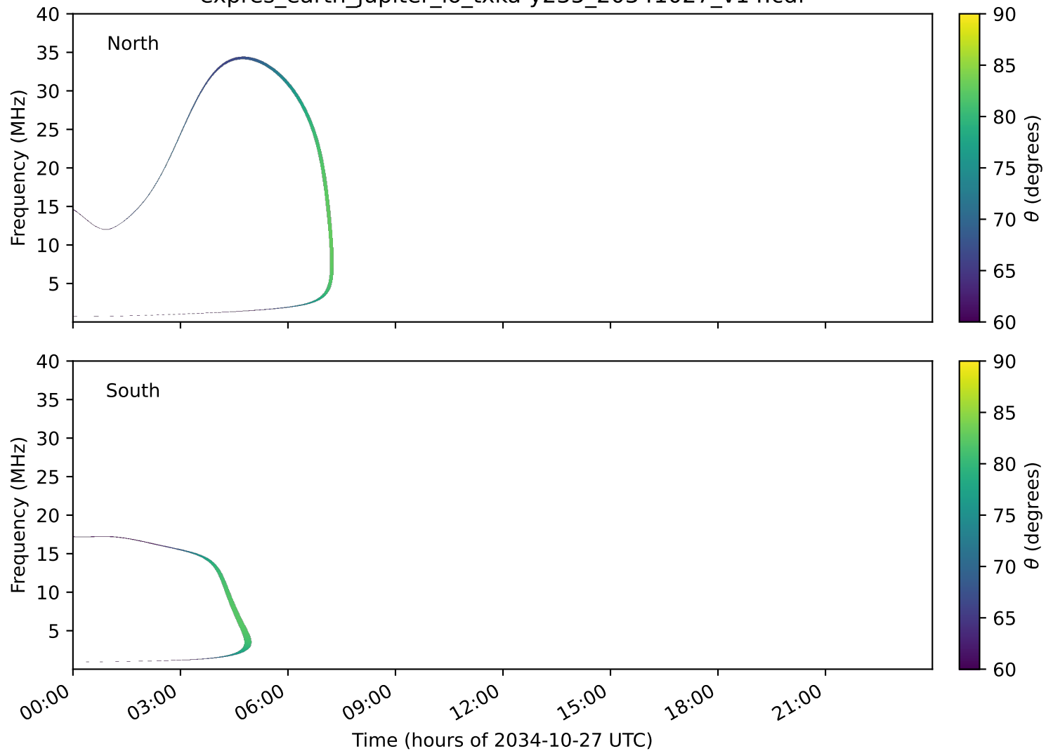
expres_earth_jupiter_io_txka-y235_20341027_v14.cdf
