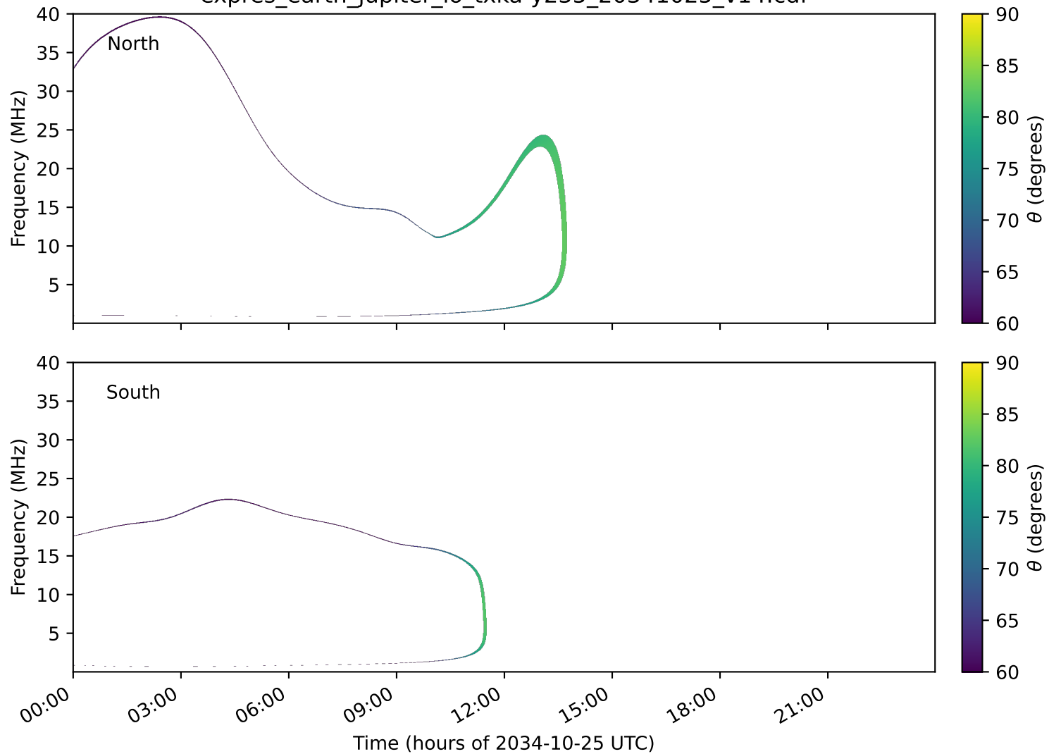
expres_earth_jupiter_io_txka-y235_20341025_v14.cdf
