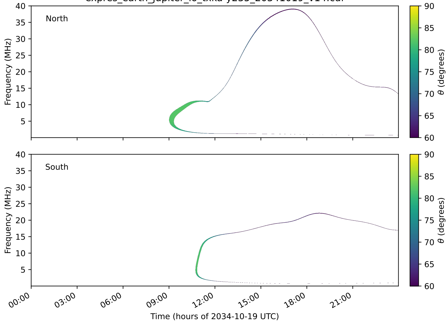
expres_earth_jupiter_io_txka-y235_20341019_v14.cdf
